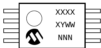
8-Lead TSSOP
